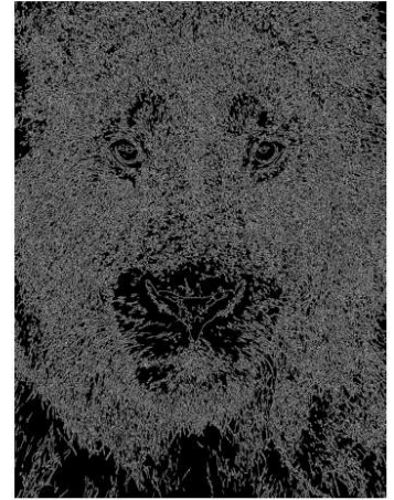
Detected Edges
